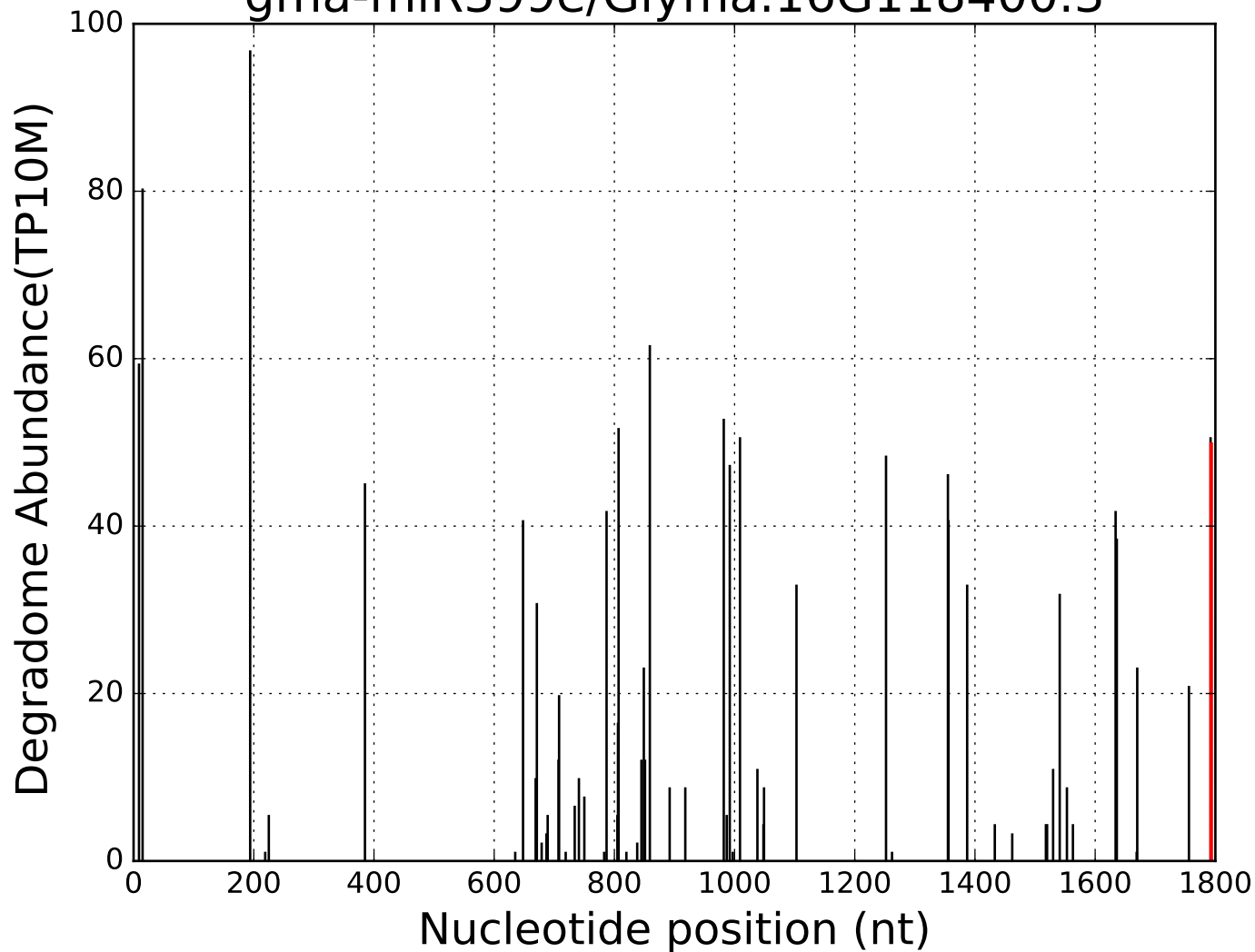
gma-miR399e/Glyma.16G118400.3
